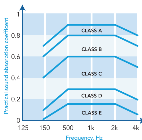
Illustration of the reference curve limiting the different sound absorption classes, from BS EN ISO 11654: 1997.
