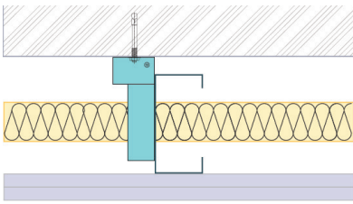
Braced Liner
