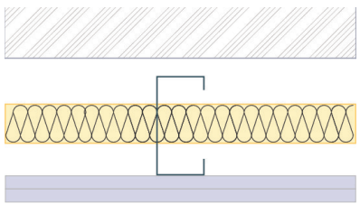
Independent Liner
