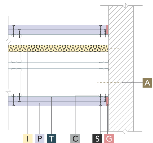
Abuttment Detail
