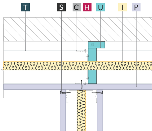
Bottom Detail
