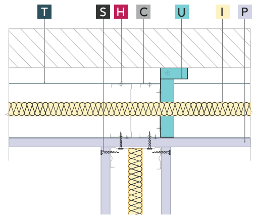
Abuttment Detail
