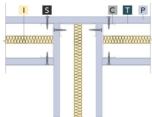
High Acoustic T - Junction Detail
